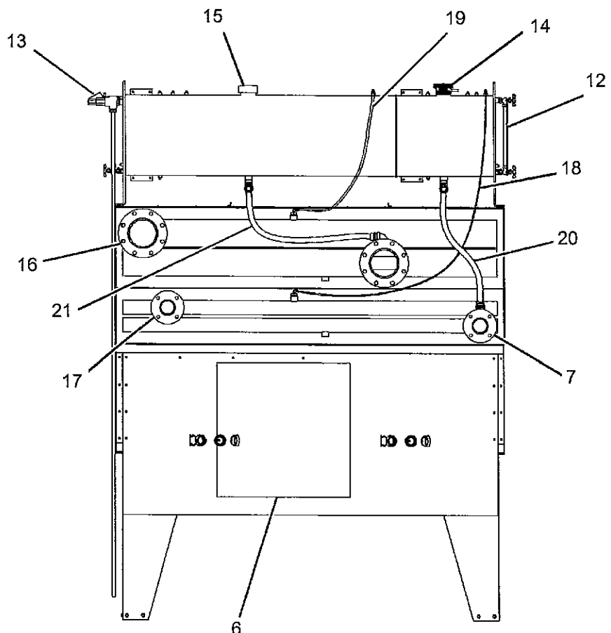
REAR VIEW
