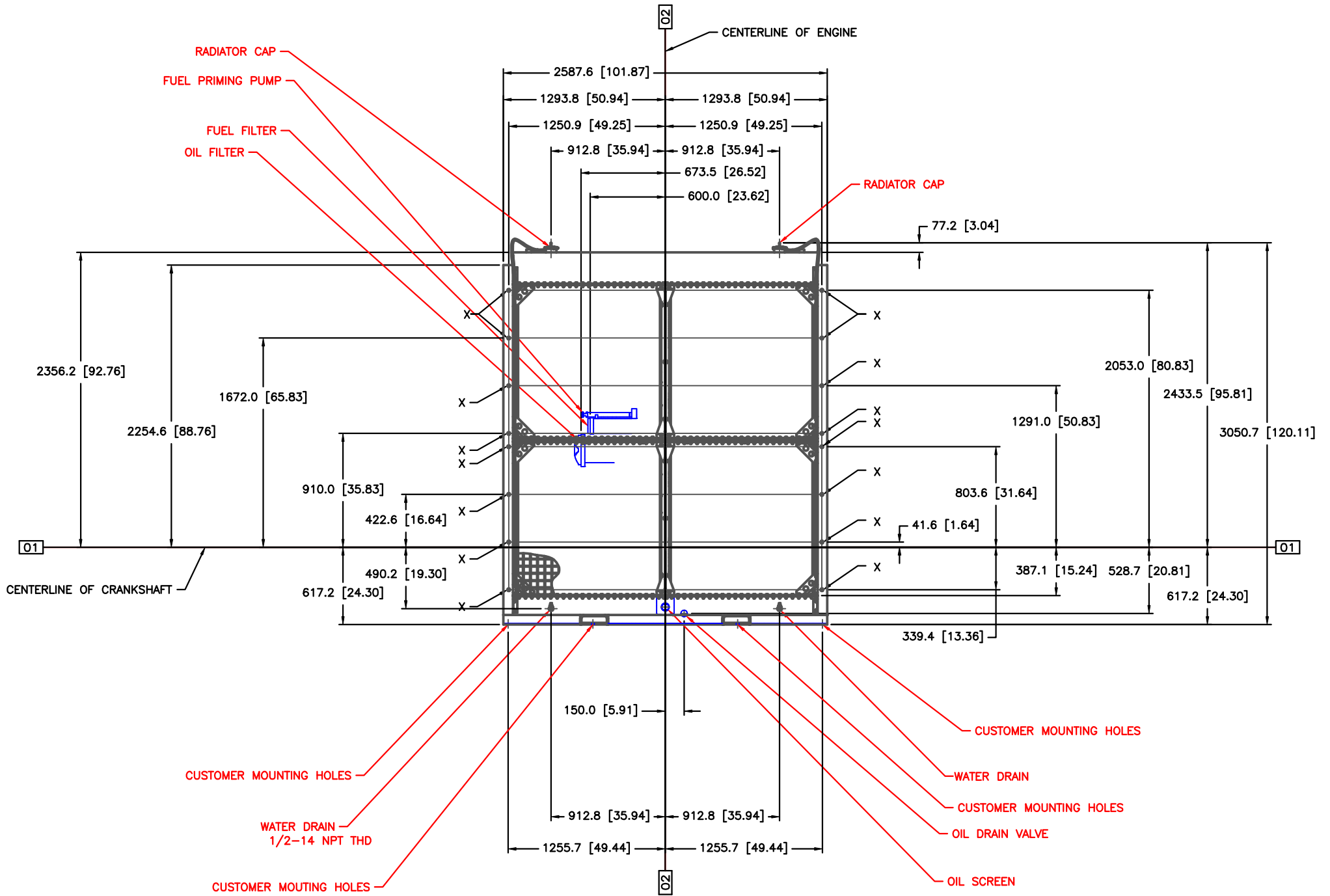
CAT 3516B PACKAGE GENERATOR SET DWG# 284-6870 CHG 00 METRIC [INCH] FRONT VIEW GP-0857 CHG 01 SHOWN
